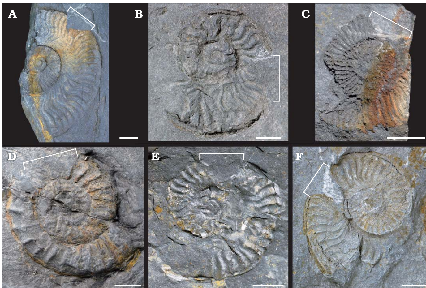
Fig. 4. Examples of early Toarcian ammonoids with ventral breakage, from the Toyora area, Japan (for detailed locality information see Fig. 2). A. Cleiviceras chrysanthemum (Yokoyama, 1904), UMUT MM 31431, loc. 8. B. Cleiviceras sp., UMUT MM 31432, loc. 5. C. Dactylioceras helianthoides (Yokoyama, 1904), UMUT MM 31433, loc. 10. D. Fontanelliceris fontanellense (Gemmellaro, 1885), UMUT MM 31434, loc. 10. E. Fuciniceris nakayamense (Matsumoto, 1947), UMUT MM 31435, loc. 3. F. Protogrammoceras onoi Hirano, 1971, UMUT MM 31436, loc. 10. The white brackets indicate the position and extent of the breakage. Scale bars 5 mm.
