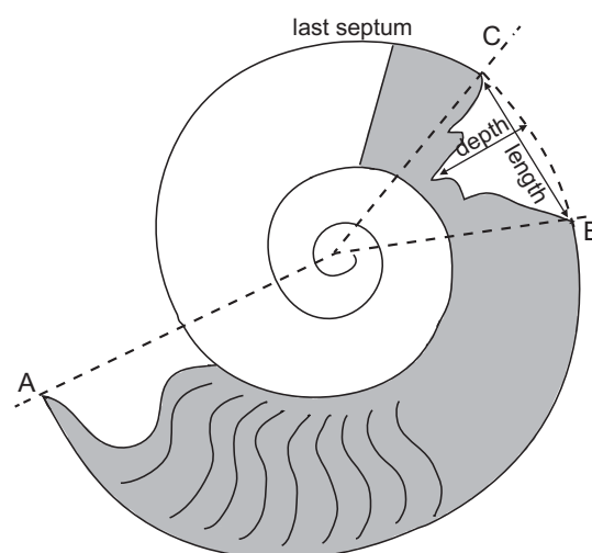
Fig. 3. Measurements for analysing the ventral breakage of ammonoid shells. Lines A, B, and C are the reference lines: A, from the coiling centre to aperture; B, apertural marginal line of damage; C, adapical marginal line of damage. Shaded area indicates body chamber. The length and depth of the breakage were also measured.
