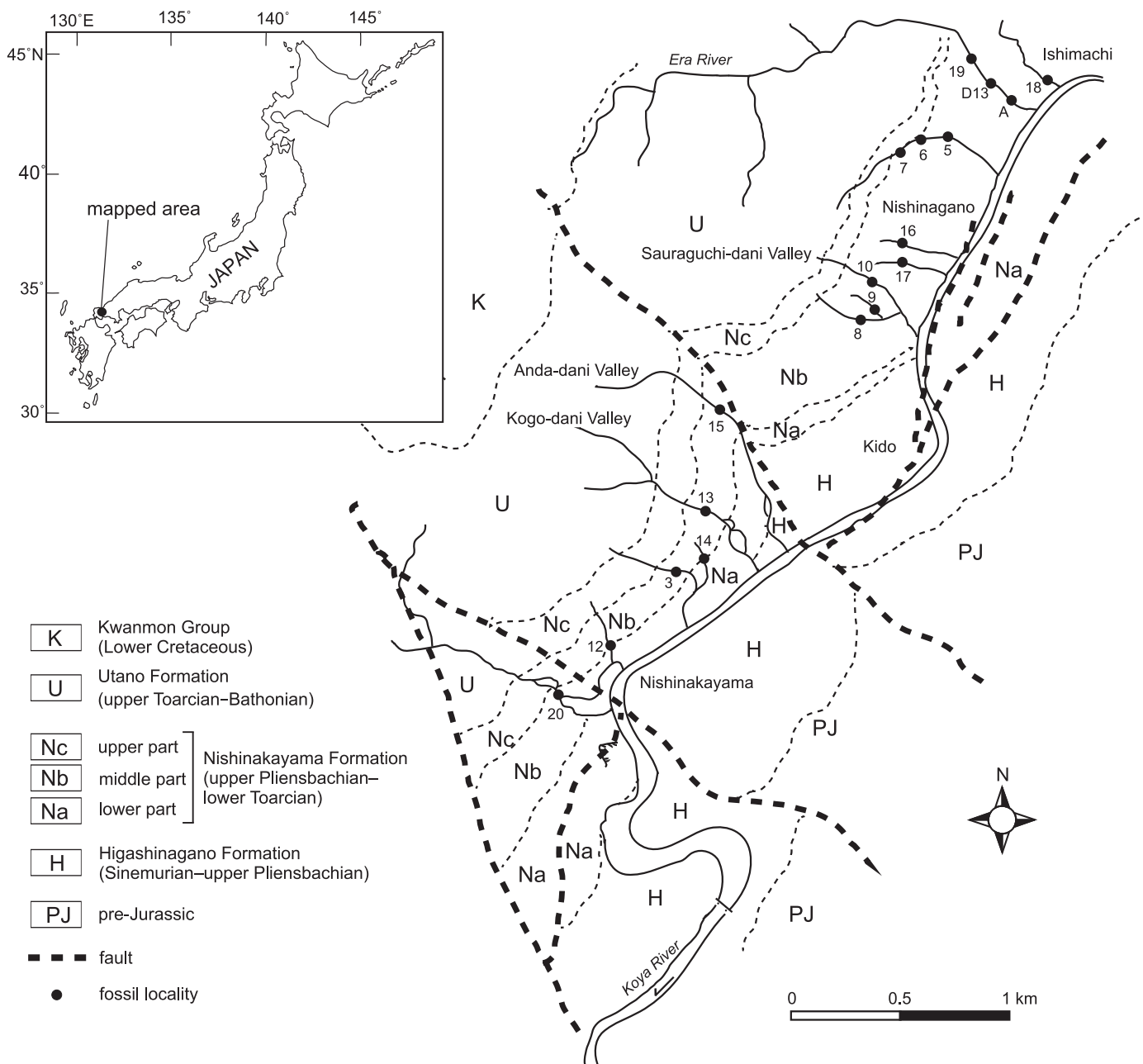
Fig. 2. Geological map of the Toyora area, southwest Japan (modified from Tanabe et al. 1982).
