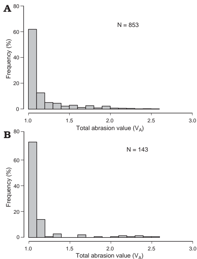
Fig. 6. Histograms of undrilled (A) and drilled (B) tests of Echinocyamus pusillus with respect to the total abrasion value. N, number of individuals.
