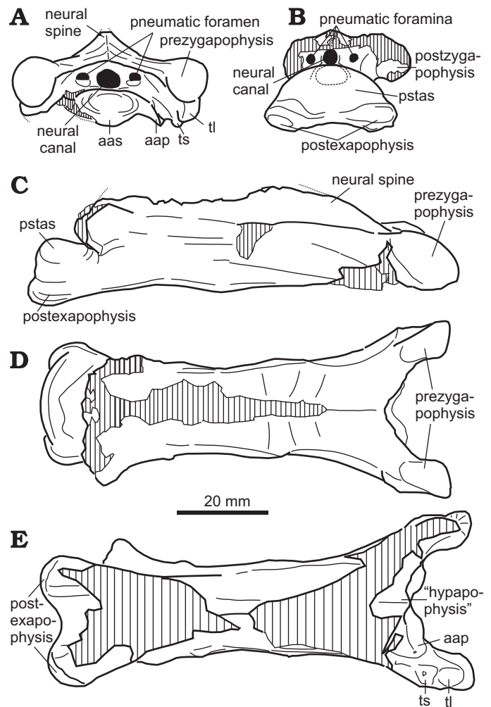
Fig. 8. Explanatory drawings of the third cervical vertebra of the Burkhanth azhdarchid (MPC-Nd 100/302) from the Upper Cretaceous of Eastern Gobi Aimag, in anterior (A), posterior (B), right lateral (C), dorsal (D), and ventral (E) views. Areas shaded with vertical lines are broken and missing. Abbreviations: aap, accessory articular process (preexapophysis); aas, anterior articular surface of the centrum; pstas, posterior articular surface of the centrum; tl and ts, large and small tubercles on the prezygapophyseal pedicle, respectively.
