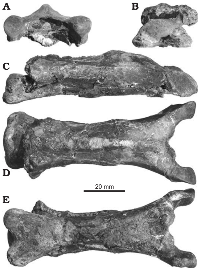
Fig. 7. Third cervical vertebra of the Burkhanth azhdarchid (MPC-Nd 100/302) from the Upper Cretaceous of Eastern Gobi Aimag, in anterior (A), posterior (B), right lateral (C), dorsal (D), and ventral (E) views.
