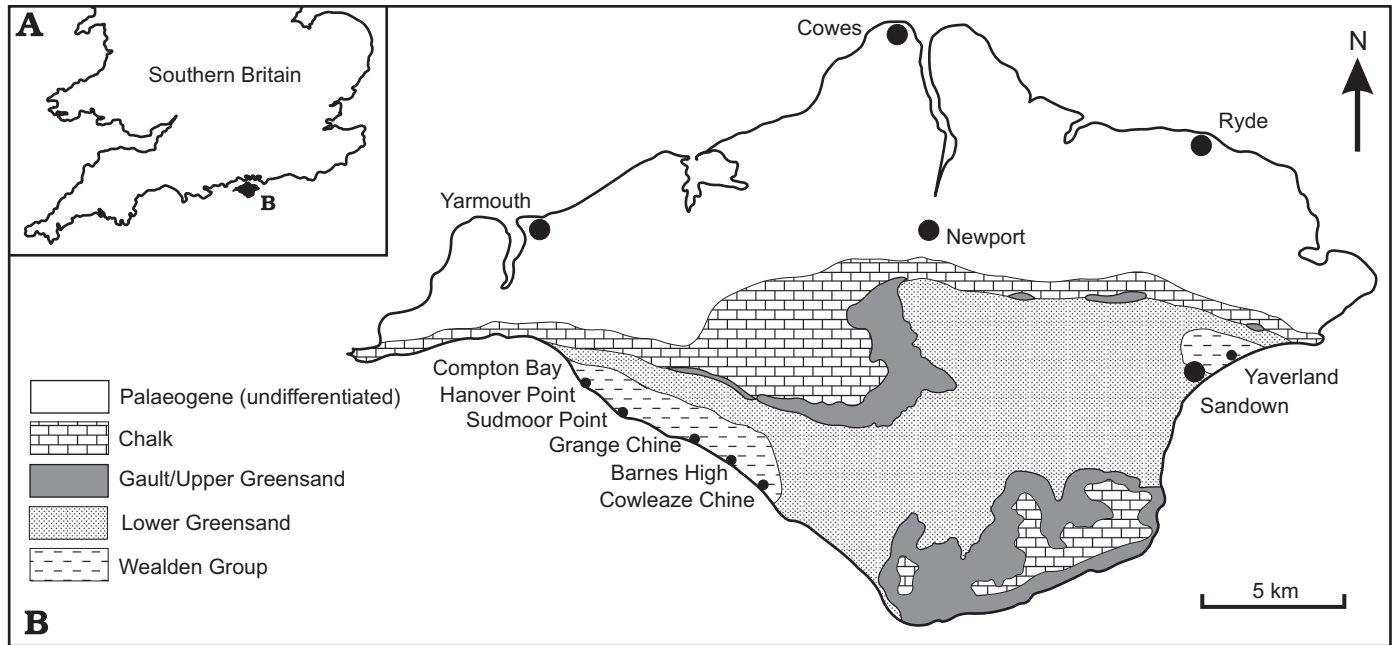
Fig. 3. A. Outline location map of Southern Britain. B. Outline geological map of the Isle of Wight.
