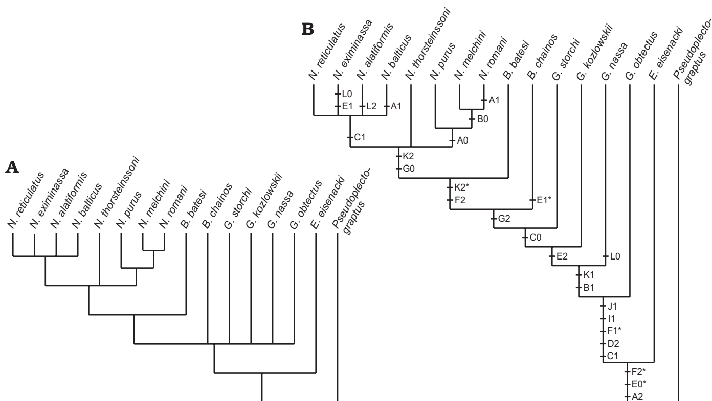
Fig. 4. Cladistic analysis. A. Our preferred of four most parsimonious trees (see text for explanation) showing positions of character state changes. Letters (characters) and numbers (states for each character) correspond to codings shown in Appendix 1. Asterisks indicate state changes to a polymorphic condition for groups of taxa above the corresponding node. B. Strict consensus tree for the cladistic analysis of the matrix shown in Appendix 2, all characters unordered and unweighted. Pseudoptograptus was used as the outgroup taxon. Tree length: 39; consistency index: 0.769; rescaled consistency index: 0.553; retention index: 0.719; homoplasy index: 0.487. Abbreviations: B. , Baculograptus ; E. , Eisenackograptus ; G. , Gothograptus ; N. , Neogothoraptus .
