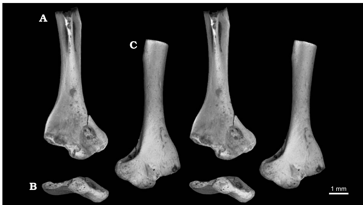
Fig. 6. Right distal humerus of eutherian group 1 (URBAC 06-062, Bissekty Formation, Upper Cretaceous: Turonian, Kyzylkum Desert, Uzbekistan), in anterior (A), distal (B), and posterior (C) views.
