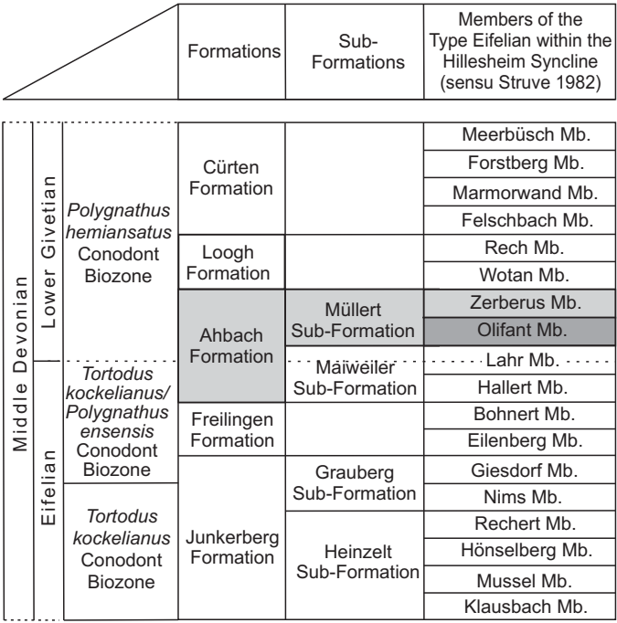
Fig. 2. Lowermost Lower Givetian stratigraphy of the “Type Eifelian Profile” sensu Struve (1982); light grey: biostratigraphic distribution of fistuliporid bryozoan Stellatoides muellertchensis gen. et sp. nov.; dark grey: maximum distribution.
