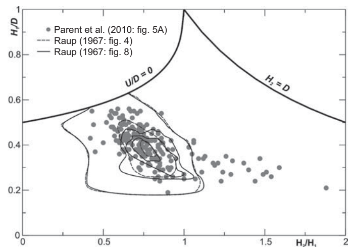
Fig. 2. Plot of a sample of 1222 observations from 201 species of Mesozoic planispiral ammonites in the morphospace ( H_2/H_1, H_1/D ), modified from Parent et al. (2010). The closed curves are the contours shown in Raup (1967: figs. 4, 8) as explained in text.
