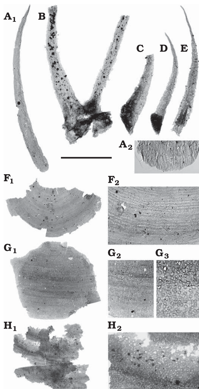
Fig. 2. Biom mineralizing taxa preserved as small carbonaceous fossils (NIGP 153954–153961) from the middle Cambrian Kaili Formation, Guizhou, China. A . Hyolithid helen (A 1 ), with detail of rounded proximal end (A 2 ), KAIL-BP-01-J38. B . Multi-rayed cancelloriid sclerite, KAIL-A-01-P39. C–E . Single-rayed or disarticulated cancelloriid sclerites. C . KAIL-GTBM-9-2-b-E39. D . KAIL-05-05-O17 (image reversed). E . KAIL-09-01-U19. F–H . Brachiopod fragments (F 1 , G 1 , H 1 ), with details of microstructure (F 2 , G 2 , G 3 , H 2 ). F . KAIL-07-01-U38. G . KAIL-05-05-E17. H . KAIL-GTBM-9-2-d-K41. Scale bars: A 1 , B–E 200 µm; A 2 40 µm; F 1 400 µm; F 2 125 µm; G 1 250 µm; G 2 125 µm; G 3 60 µm; H 1 500 µm; H 2 150 µm.
