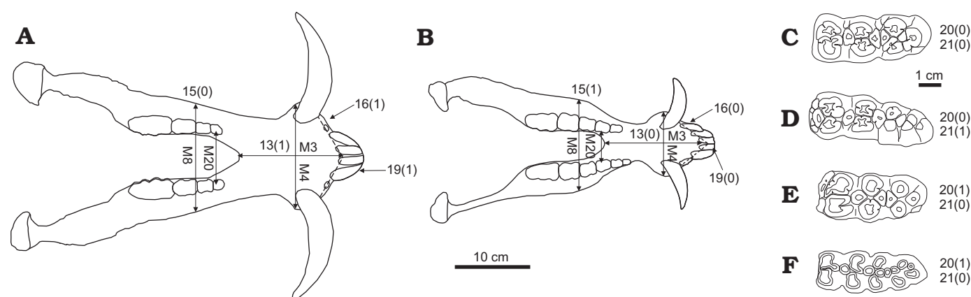
Mandibular and dental character states. Mandibles (A, B) and lower third molars (C–F) are schematically represented in dorsal and occlusal views, respectively. A . Hylochoerus meinertzhageni , male (MRAC 17783). B . Potamochoerus sp., male (MNHN-ZM-AC, no number). C . Kolpochoerus limnetes (OMO 18-1968-2104). D . Kolpochoerus limnetes (OMO 354-10004). E . Kolpochoerus majus (KL 251-2). F . Hylochoerus meinertzhageni (MNHN-ZM-AC 1951-208). Characters 14 and 17 are coded in the same way as characters 13 and 16, respectively, but on female specimens. Mandibular measurements used to code characters are illustrated.
