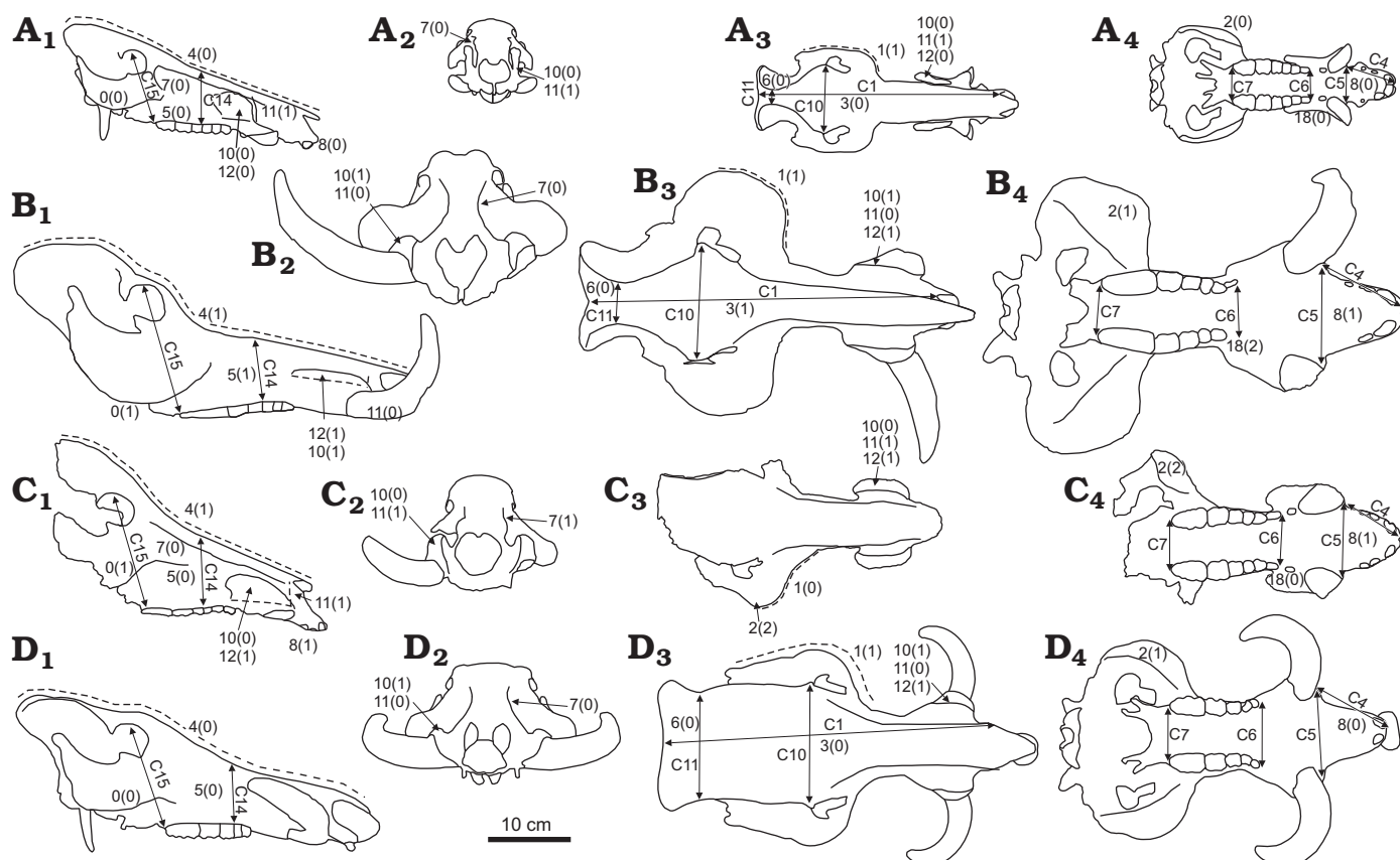
Cranial character states. Each cranium is schematically represented in lateral (1), anterior (2), dorsal (3), and ventral (4) views. A . Potamochoerus larvatus (MRAC 920). B . Kolpochoerus olduvaiensis (KNM-ER 788). C . Kolpochoerus phillipi sp. nov. (MAT-VP-1/5). D . Hylochoerus meinertzhageni (MRAC 17783). All specimens are males. Character 9 is coded in the same way as character 8, but on female specimens. Cranial measurements used to code characters are illustrated.
