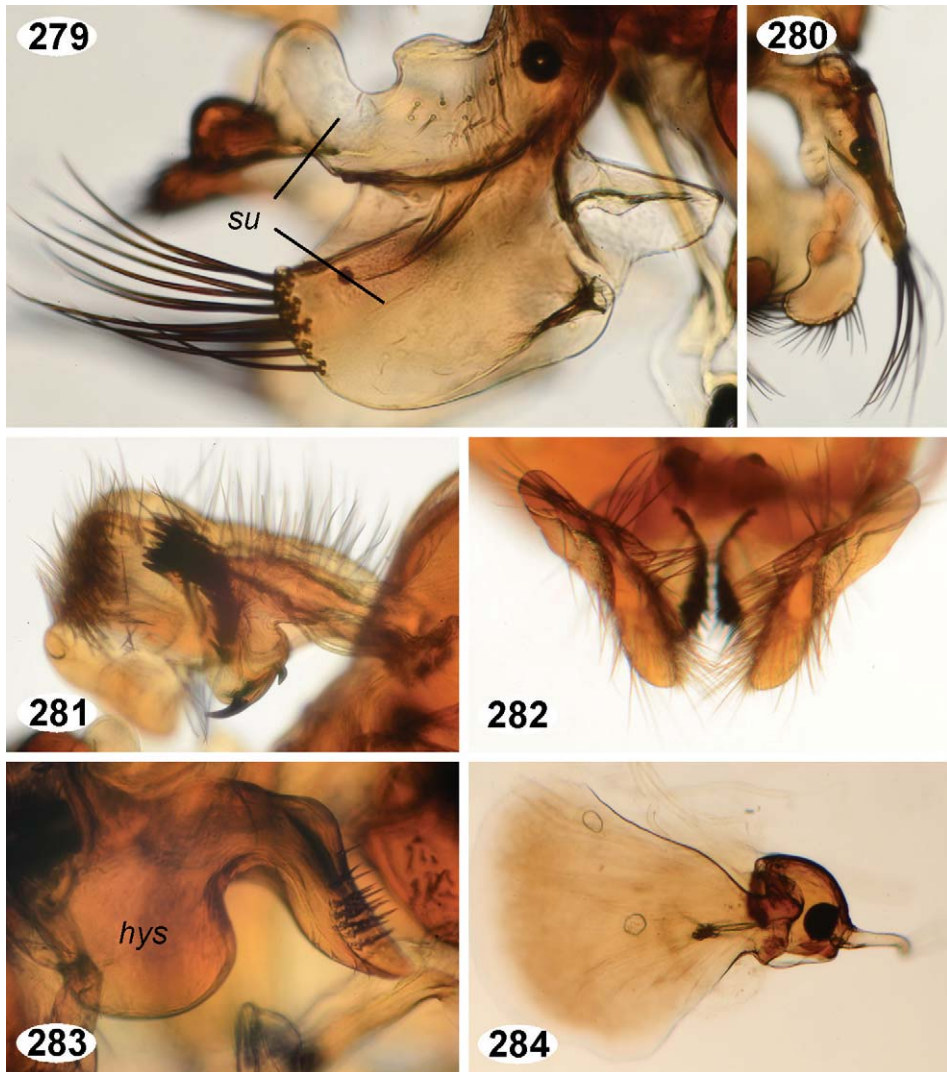
Figs 279–284. Terminalia (♂) of Stylogaster spinicercus sp. n. (holotype): (279) surstylus, lateral view; (280) same, dorsal view; (281) cercus, lateral view; (282) same, ventral view; (283) phallus sheath of hypandrium, lateral view; (284) sperm pump and ejaculatory apodeme. Abbreviations: hys – phallus sheath of hypandrium; su – surstylus. Not to scale.
