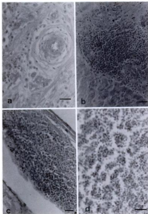
FIGURE 2. Inflammatory lesions in a red fox with Borrelia spp. infection, Sapporo, Hokkaido, Japan, June 1992. H&E stain. Each bar = 10 µm. a. Skin lesion without tick bite; spirochetes were isolated from the site; b. Perivascular cell infiltration and hepatitis in the liver; c. Pyelitis; d. Conjunctivitis.
