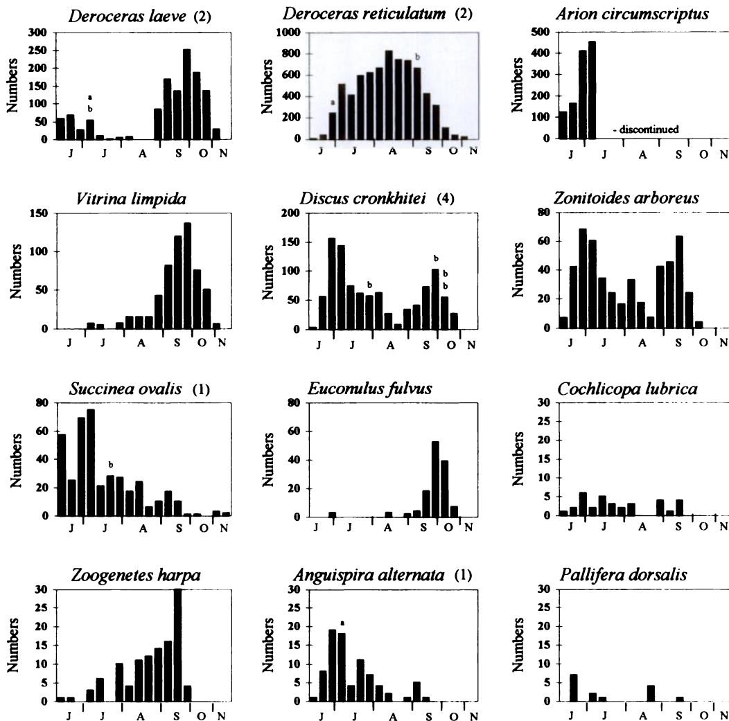
FIGURE 1. Twelve species of terrestrial gastropods collected from beneath 200 cardboard sheets from 15 June to 25 November 1994, near Grand Marais, Minnesota. Numbers of each species infected with Parelastrongylus tenuis are in brackets. Those gastropods containing first- or second-stage P. tenuis larvae are indicated by a ; those with third-stage larvae by b . Letters on x-axis refer to June (J), July (J), August (A), September (S), October (O), and November (N).
