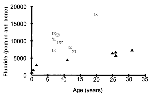
FIGURE 2. Relationship of age (years) and rib fluorine (F) content (ppm F in bone ash) for beluga whales sampled in Hudson Bay (□) and in the St. Lawrence Estuary (▲).
