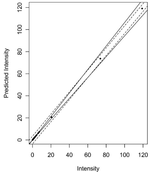
FIGURE 3. Estimated hematozoan intensity 95% confidence bounds using standard errors from mean field:image ratios for 10 slides (solid line, SE=0.18) and mean difference between manually and digitally quantified intensity (dashed line, SE=1.71). Confidence bounds intersect at intensity=58. Points represent intensity of hematozoan infection from examined blood smears ( n=32 ).
