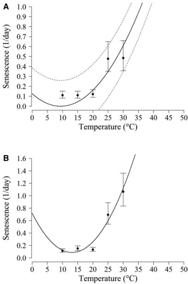
Fig 4. Temperature-dependent senescence rates (day 1) for L. huidobrensis adult females (A) and males (B). Fitted curves of senescence rates: Ratkowski-1 model (solid line). Bars represent standard deviation of the median senescence rate.
