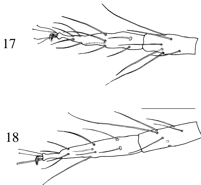
FIGURES 17-18: Tetranychus arifi sp. nov. (showing female tarsi and tibiae) 17. Leg III; 18. Leg IV (100 µm).
