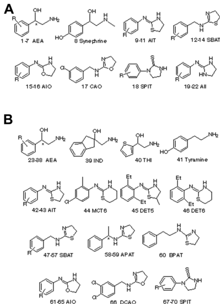
Figure 1. Structures of octopamine agonists used for regression analysis in study (a) and test (b) sets.
