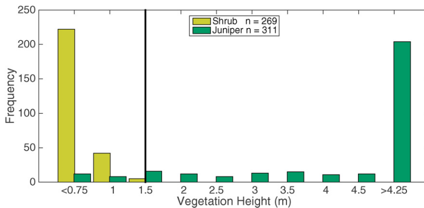
Figure 3. Histogram of measured vegetation heights of junipers and shrubs. The vertical black line shows the 1.5 m cutoff used in this study to classify junipers.
