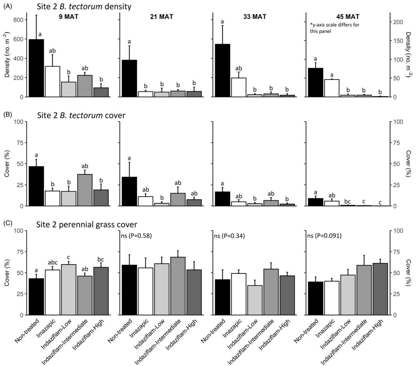
Figure 2. Mean (+1 SE) Bromus tectorum density (A), B. tectorum cover (B), and perennial grass cover (C) at Site 2 (Half Moon) at 9, 21, 33, and 45 mo after treatment (MAT; cover = absolute canopy cover). Herbicide treatments were applied in September 2016 when native plants were dormant and B. tectorum was 100% post-seed set. Letters indicate significant within-year differences among treatment means (Tukey’s honest significant difference, \alpha = 0.05 , n = 4 ). Herbicide treatments are as follows: imazapic = imazapic 123 g ai ha -1 ; indaziflam-low = indaziflam 44 g ai ha -1 ; indaziflam-intermediate = indaziflam 73 g ai ha -1 ; indaziflam-high = indaziflam 102 g ai ha -1 . All treatments included a 0.25% v/v nonionic surfactant. Note that y-axis scale is consistent across panel rows in all cases, except for B. tectorum density at 45 MAT (*).
