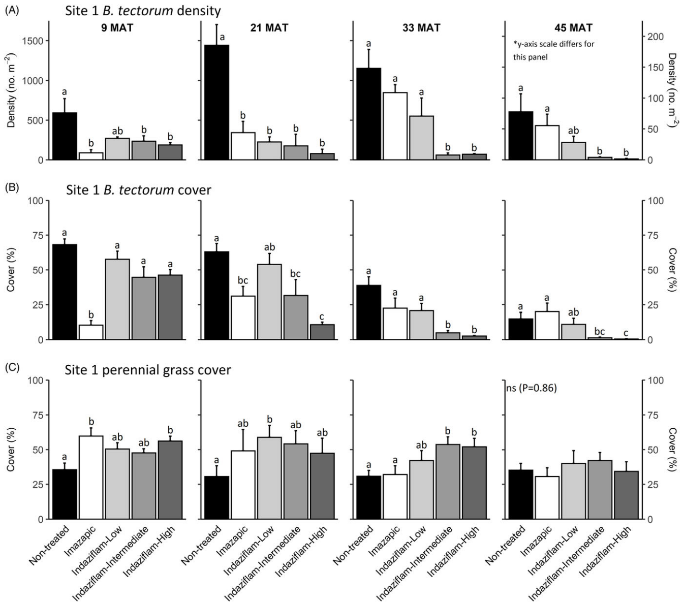
Figure 1. Mean (+1 SE) Bromus tectorum density (A), B. tectorum cover (B), and perennial grass cover (C) at Site 1 (Boulder Lake) at 9, 21, 33, and 45 mo after treatment (MAT; cover = absolute canopy cover). Herbicide treatments were applied in September 2016 when native plants were dormant and B. tectorum was 100% post-seed set. Letters indicate significant within-year differences among treatment means (Tukey's honest significant difference, \alpha = 0.05 , n = 4 ). Herbicide treatments are as follows: imazapic = imazapic 123 g ai ha -1 ; indaziflam-low = indaziflam 44 g ai ha -1 ; indaziflam-intermediate = indaziflam 73 g ai ha -1 ; indaziflam-high = indaziflam 102 g ai ha -1 . All treatments included a 0.25% v/v nonionic surfactant. Note that y-axis scale is consistent across panel rows in all cases, except for B. tectorum density at 45 MAT (*).
