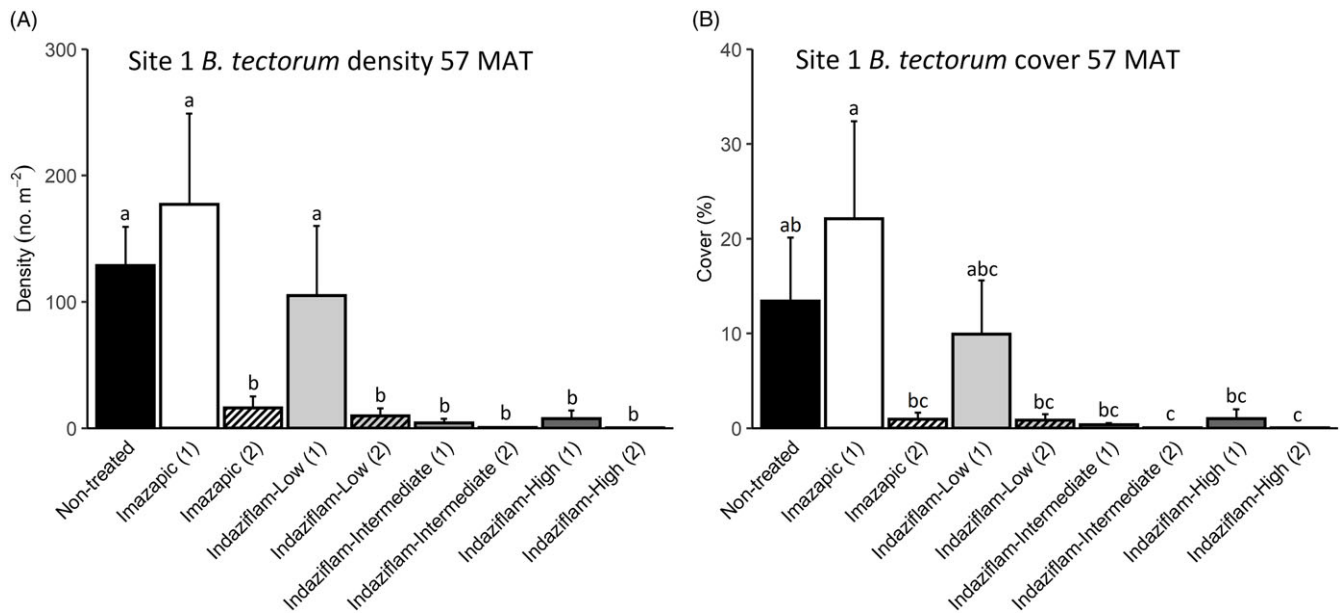
Figure 3. Mean ( \pm 1 SE) Bromus tectorum density (A) and B. tectorum cover (B) at Site 1 (Boulder Lake) at 57 mo after treatment (MAT; cover = absolute canopy cover). Treatment groups followed by a (1) received only one herbicide application, and treatment groups followed by a (2) received a sequence of two herbicide applications (diagonal line pattern). Initial herbicide treatments were applied in September 2016, and reapplications of the same treatments were made approximately 45 mo later in June 2020. Native plants were dormant and B. tectorum was 100% post-seed set when initial treatments were applied, and native plants were actively growing and B. tectorum was near 100% post-seed set when reapplication occurred. Letters indicate significant differences among treatment means (Tukey's honest significant difference, \alpha = 0.05 , n = 4 ). Herbicide treatments are as follows: imazapic = imazapic 123 g ai ha -1 ; indaziflam-low = indaziflam 44 g ai ha -1 ; indaziflam-intermediate = indaziflam 73 g ai ha -1 ; indaziflam-high = indaziflam 102 g ai ha -1 . All treatments (initial and reapplication) included a 0.25% v/v nonionic surfactant.
