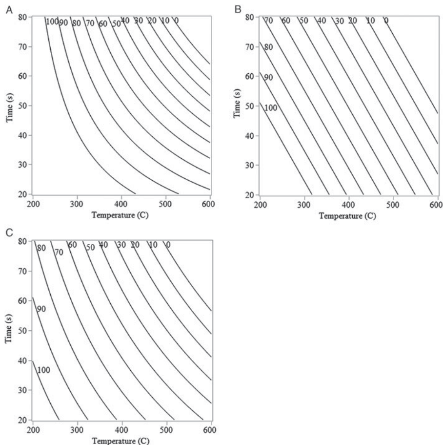
Figure 2. Contour maps for (A) sicklepod, (B) velvetleaf, and (C) hemp sesbania survival after exposure to various temperature and heating periods in a high-fire kiln at the Alzheimer Laboratory in Fayetteville, AR.
