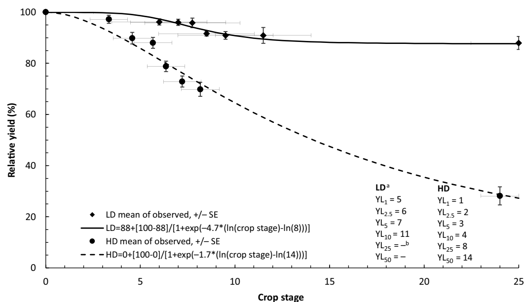
Figure 4. Relative corn yield as a function of crop stage at the time of herbicide application. Nine experiments, conducted at Ridgetown Campus, Ridgetown, ON (2017–2019) and the Huron Research Station, Exeter, ON (2017–2018), were separated into two groups, lower (LD, 12 to 82 weeds m -2 ) and higher (HD, 132 to 411 weeds m -2 ) weed densities. Predicted regression lines were calculated using the log-logistic model (Equation 1). LD ME = 0.4, RMSE = 4.7; HD ME = 0.78, RMSE = 12.1. a YL 1 , YL 2.5 , YL 5 , YL 10 , YL 25 , and YL 50 : crop stage at the application that led to a 1%, 2.5%, 5%, 10%, 25%, and 50% yield loss in corn, relative to the season-long weed-free control. b Non-estimable. c Sequential numeric values assigned to vegetative and reproductive corn stages: 0 = preemergence, 1 = V1... 17 = V17, 24/25 = R7. ME, modeling efficiency; RMSE, root mean square error.
