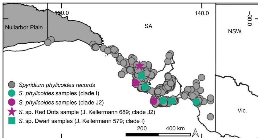
Fig. 4. Distributions of samples of S. phyllicoides , S. sp. Red Dots (J. Kellermann 689) and S. sp. Dwarf (J. Kellermann 579) used in this study. For S. phyllicoides , samples are coloured by the clades in which they are placed in the nrDNA tree (Fig. 2), with the distribution of the species, on the basis of the records in the Atlas of Living Australia (2020), also shown (grey dots).
