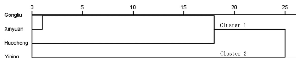
Figure 3. Cluster analysis performed with the pollen metrical variables from 4 groups of wild apricots ( Prunus armeniaca ).
