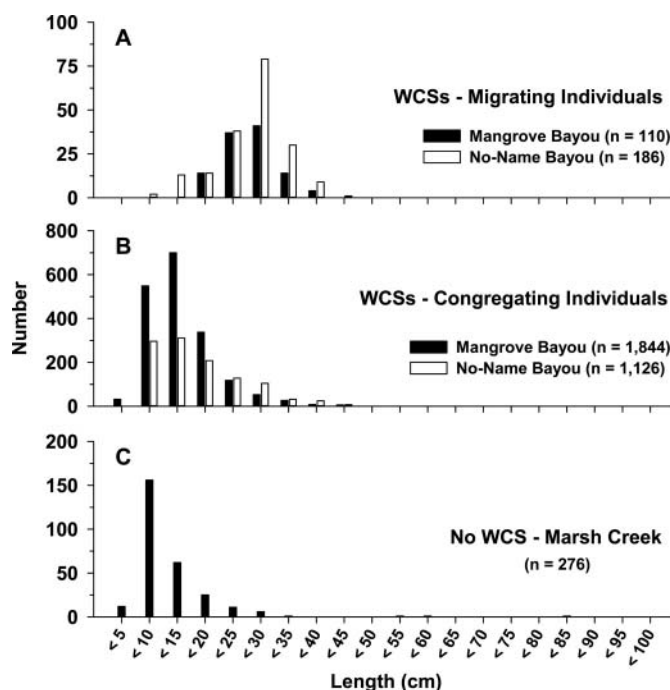
FIGURE 3. Length-frequency distribution for nekton observed with dual-frequency identification sonar at three sites in the Calcasieu Lake estuary: (A) migrating individuals ( n = 296 ) at each water control structure (WCS), (B) congregating individuals ( n = 2,970 ) at each WCS, and (C) individuals ( n = 276 ) at the salt-marsh creek (no WCS). Note that the y-axis scale differs among the panels.
