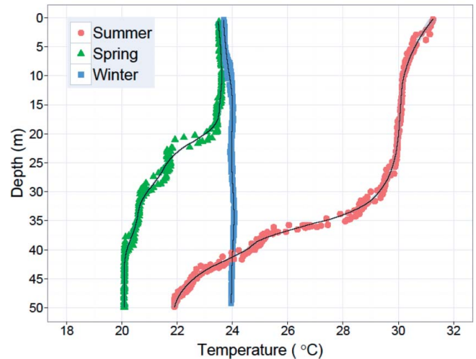
FIGURE 3. Temperature versus depth data collected on the day of tagging for each seasonal trial using a Manta2 water quality multiprobe at oil and gas platform site MU-762-A (water depth of 50 m). The black smoothing lines were fitted to the temperature data using a Loess model.
