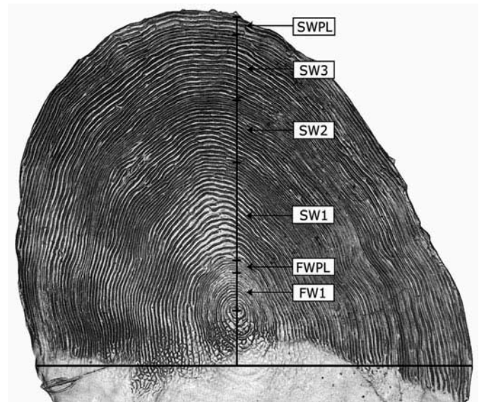
FIGURE 3. Scale image from an age-1.3 Sockeye Salmon showing the reference line used to measure growth and growth zones. The growth indices used in the analysis include the freshwater scale radius (FWSR = FW1 + FWPL) and the scale radius to the end of the first year at sea (L1SR = FW1 + FWPL + SW1).
