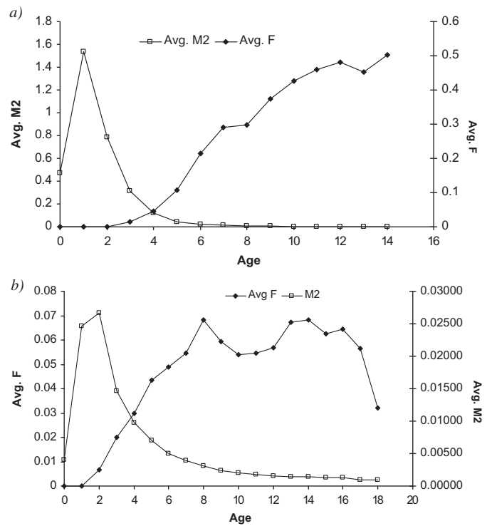
FIGURE 7. Average (1990–2007) predation mortality ( M_2 ) at age and average (1990–2007) fishing mortality ( F ) at age for (a) Hoki and (b) Southern Blue Whiting in the southern Chilean demersal fishery.
