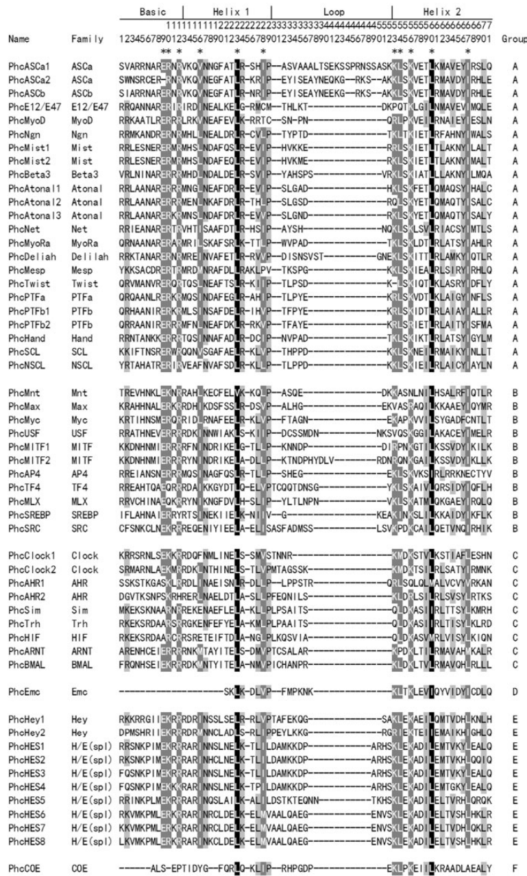
Fig. 1. Multiple alignment of the 55 PhcbHLH motifs. Highly conserved sites are marked with asterisks and hyphens denote gaps. The family names and high-order groups have been organized according to Table 1.
