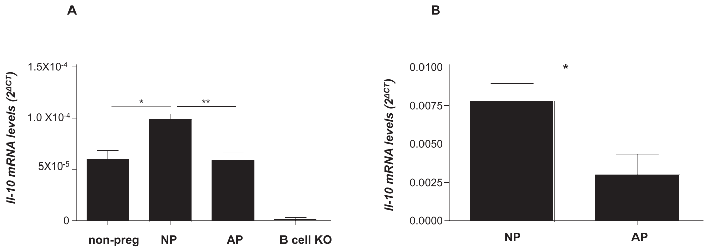
FIG. 2 IL-10 expression is augmented in normal pregnancies. A) IL-10 mRNA expression is augmented in the spleen of NP mice compared to that of AP and non-preg mice. As a further control, we analyzed the expression of IL-10 in the spleen of B cell knockout females (B cell KO). B) CD19 + B cells were isolated either from NP or from AP mice and further stimulated in vitro with LPS + PMA + iono for 5 h. Stimulated CD19 + B cells isolated from NP mice showed a significantly higher expression of IL-10 mRNA compared to B cells isolated from AP mice. Data are expressed as mean ± SEM. * P < 0.05, ** P < 0.01, as analyzed by one-way ANOVA, followed by Tukey multiple-comparison test.
