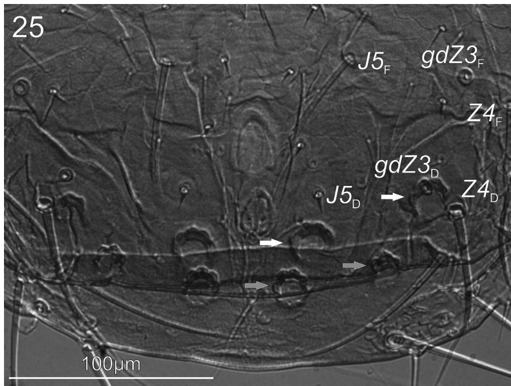
FIGURE 25. Zircon hamaricus sp. nov., opisthonotum of deutonymph moulting to female. D in subscript – deutonymph characters, F in subscript – female characters, white arrows – female’s posterodorsal cavities, gray arrows – deutonymph’s posterodorsal cavities.
