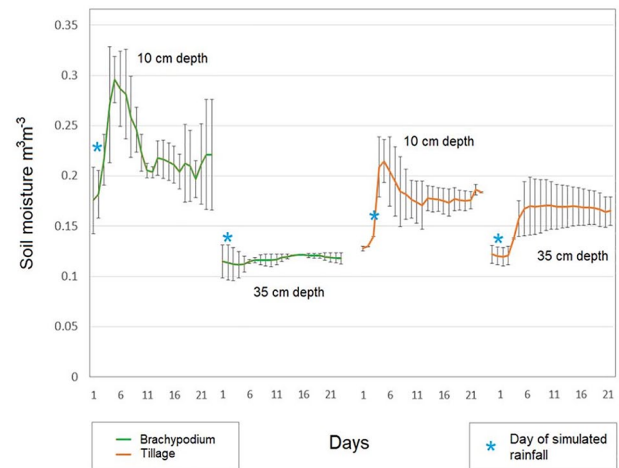
Figure 5. Evolution of volumetric soil moisture at 10 and 35 cm depth in Brachypodium distachyon and tillage treatments. Average of 3 plots during 20 days after the simulation in the late autumn. Bars represent standard deviation.
