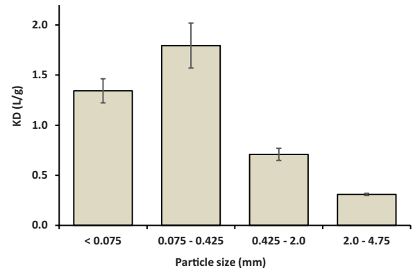
Figure 4. Effect of particle size on phosphate adsorption onto pumice.
