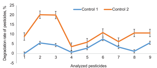
Figure 7. A comparison of the degradation rate of obsolete pesticides in control 1 (unimproved soil) and 2 (improved soil), in 3 months. 1: β-BHC; 2: Heptachlor-epox pure; 3: Dieldrin; 4: Endrin aldehyde; 5: β-Endosulfan; 6: δ-BHC; 7: Heptachlor; 8: Aldrin; 9: α-Endosulfan; values are in mean ± SD, n=3. Values with different letters are statistically significantly different at P \leq .05 .
