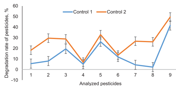
Figure 8. A comparison of the degradation rate of obsolete pesticides in control 1 (unimproved soil) and control 2 (improved soil) in 6 months. 1: β-BHC; 2: Heptachlor-epox pure; 3: Dieldrin; 4: Endrin aldehyde; 5: β-Endosulfan; 6: δ-BHC; 7: Heptachlor; 8: Aldrin; 9: α-Endosulfan; values are in mean ± SD, n=3. Values with different letters are statistically significantly different at P \leq .05 .
