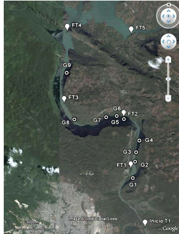
Fig. 3. Locations where spider monkey subgroups were detected along the river canyon. White circles with the "G" and a number indicate the identity of the subgroup. Image modified after Google Earth.
