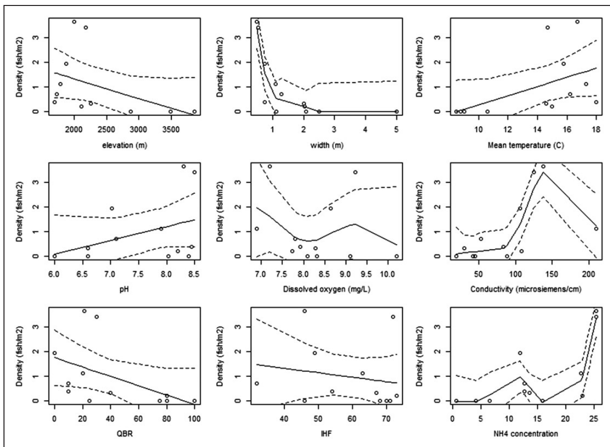
Figure 5. Smoothed curve of the additive effect of individual environmental parameters on estimated Astroblepus vaillanti abundance ( \text{fish m}^{-2} ) using Generalized Additive Models (GAMs). Dotted lines represent 95% confidence intervals.
