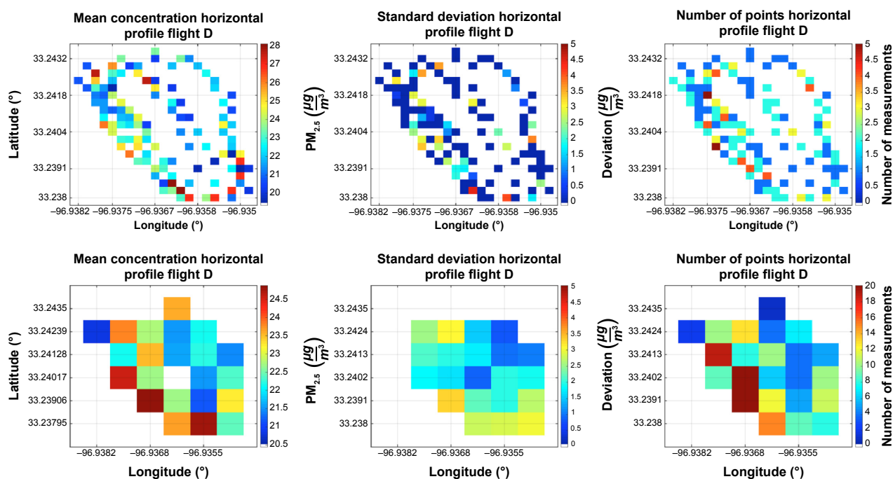
Figure 8. Mean \text{PM}_{2.5} concentration, standard deviation, and number of measurements for Flight D divided into 30 \text{ m} \times 15 \text{ m} (top) and 120 \text{ m} \times 65 \text{ m} (bottom) grids.
