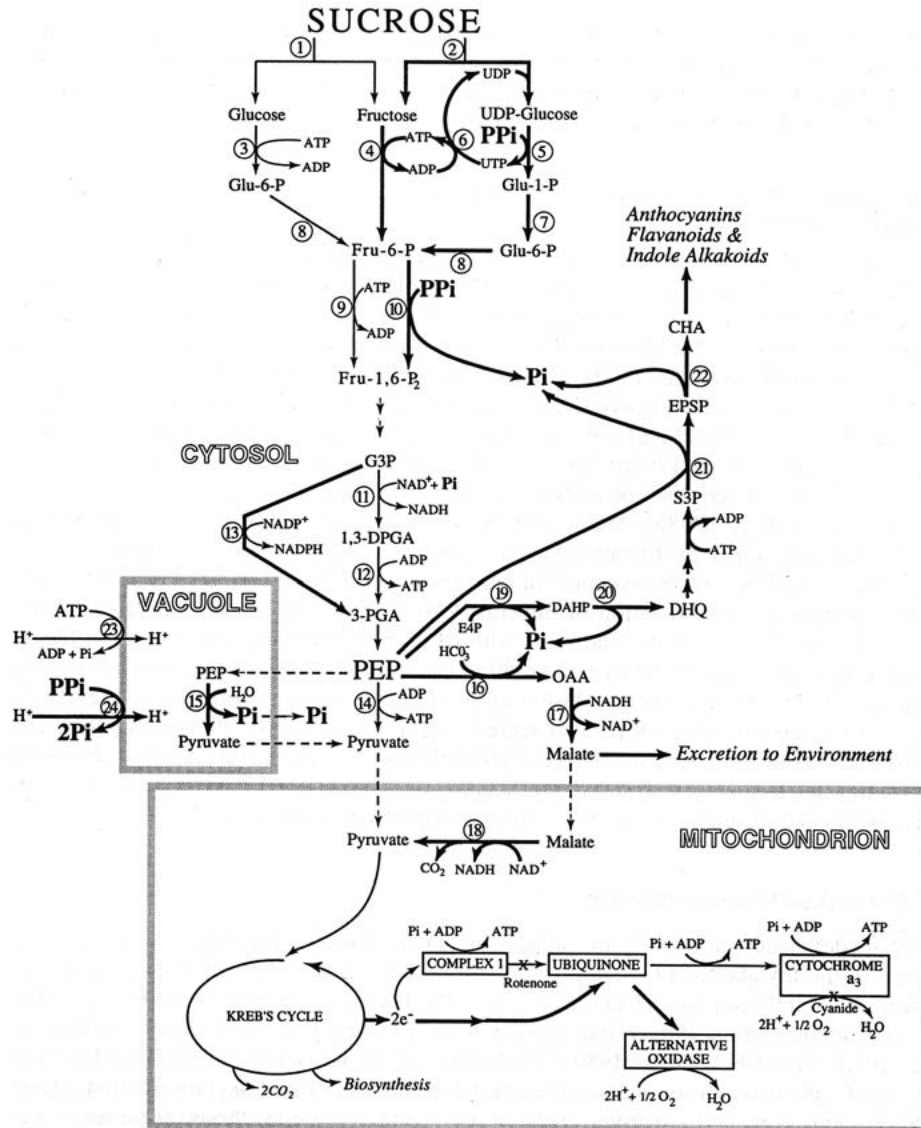
Fig.14. Model indicating several changes in plant metabolism occurring in response to Pi deficiency. The modified pathways are indicated with bold arrows. The enzymes that catalyze the numbered reactions are: 1, invertase; 2, sucrose synthase; 3, hexokinase; 4, fructokinase; 5, UDP-glucose pyrophosphorylase; 6, nucleoside diphosphate kinase; 7, phosphoglucomutase; 8, phosphoglucose isomerase; 9, ATP-dependent phosphofructokinase; 10, pyrophosphate-dependent phosphofructokinase; 11, NAD-dependent glyceraldehyde 3-phosphate dehydrogenase (phosphorylating); 12, 3-phosphoglycerate kinase; 13, NADP-dependent glyceraldehyde 3-phosphate dehydrogenase (non-phosphorylating); 14, pyruvate kinase; 15, phosphoenolpyruvate phosphatase; 16, phosphoenolpyruvate carboxylase; 17, malate dehydrogenase; 18, malic enzyme; 19, 3-deoxy-D-arabino-heptulosonate-7-phosphate (DAH) synthase; 20, 3-dehydroquininate dehydratase; 21, 5-enolpyruvylshikimate 3-phosphate (EPSP) synthase; 22, chorismate synthase; 23, tonoplast H + -ATPase; 24, tonoplast H + -pyrophosphate. Abbreviations are as follow: CHA, chorismate; DAHP, 3-deoxy-D-arabino-heptulosonate-7-phosphate; DHQ, dehydroquininate; 1,3-DPGA, 1,3-diphosphoglycerate; E4P, erythrose 4-phosphate; EPSP, 5-enolpyruvylshikimate 3-phosphate; Fru-6-P, fructose 6-phosphate; Fru-1,6-P 2 , fructose 1,6-bisphosphate; Glu-1-P, glucose 1-phosphate; Glu-6-P, glucose 6-phosphate; G3P, glyceraldehyde 3-phosphate; G3PDH, glyceraldehyde 3-phosphate dehydrogenase; OAA, oxaloacetate; PEP, phosphoenolpyruvate; 3-PGA, 3-phosphoglycerate; PPI, pyrophosphate; S3P, shikimate 3-phosphate. Reproduced from Plaxton and Carswell (1999) with permission by Marcel Dekker Inc.
