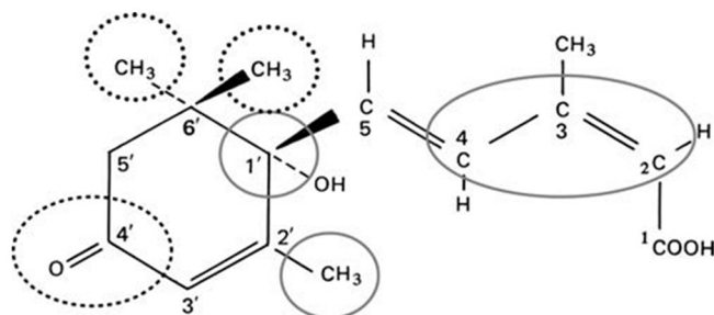
Figure 2. Structure of ABA.
