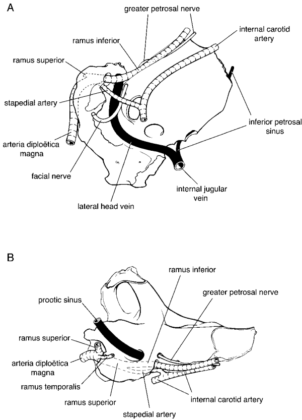
Fig. 3. Reconstruction of major arteries, veins, and nerves on the right petrosal referred to Prokennalestes trofimovi , PSS-MAE 136. A , Ventral view. B , Lateral view.
