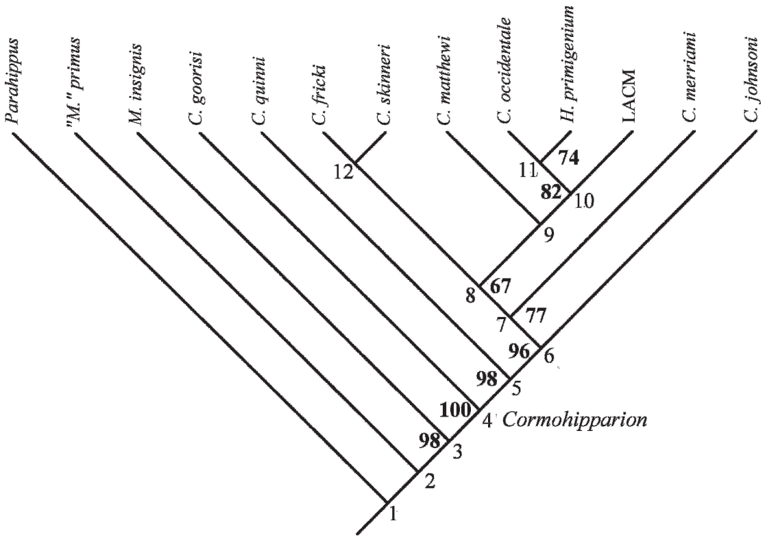
Fig. 30. Cladogram of species of Cormohipparion , the LACM specimen, and Hipotherium primigenium with outgroups of Parahippus leonensis , " Merychippus " primus , M. insignis . Tree length is 124; Consistency Index is 0.742; Retention Index is 0.782; Homoplasy Index is 0.258. Bootstrap values are in boldface. Based on a character distribution analysis via MacClade 4.08. Nodes 1–8 are as in fig. 27.
