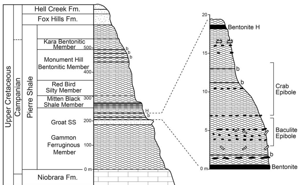
FIGURE 3. Stratigraphic section of the Pierre Shale at AMNH loc. 3296 showing the baculite and crab epiboles (modified after Bishop, 1985a). Abbreviation: b , bentonite.
