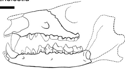
zhelestid
