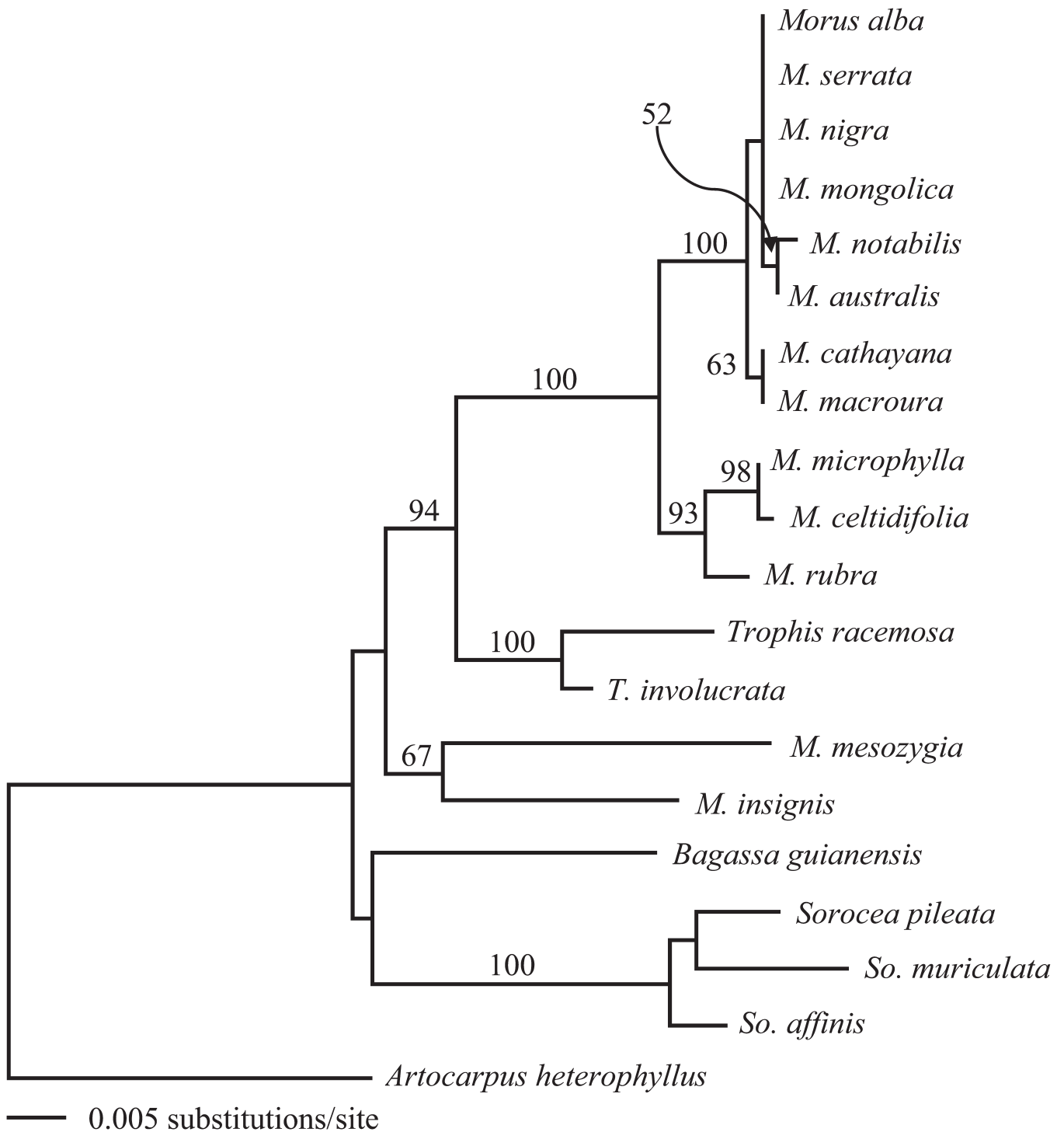
FIG. 3. Maximum Likelihood phylogram (-Ln likelihood = 4,700.73975, the most likely tree) based on the combined data set using a K81uf + G evolutionary model. Numbers above the branches are ML bootstrap values based on 1,000 replicates.
