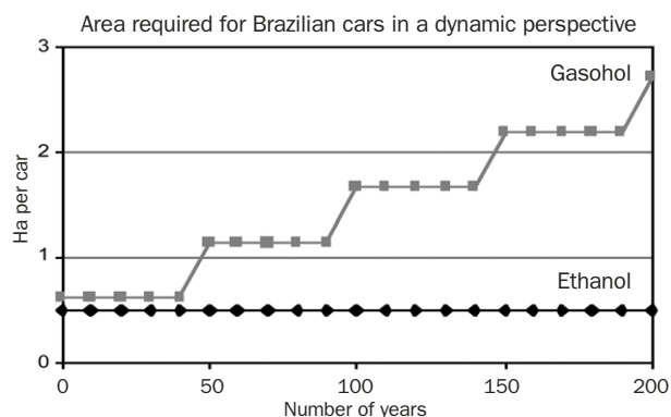
Figure 1. The footprint of Brazilian ethanol and gasoline in a dynamic perspective.
