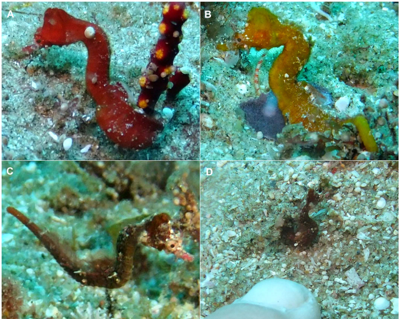
Fig. 4. Cylix nkosi in situ, 2 Mile Reef, Sodwana Bay, KwaZulu-Natal, South Africa, 22 m depth: (A) male, pregnant, red coloration; (B) male, pregnant, yellow coloration; (C) female, brown coloration; (D) female, brown coloration. Photographs © Christo van Jaarsveld (SeaXplore), used with permission.
