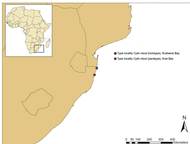
Fig. 5. Distribution of Cylix nkosi in South Africa. Red dot = type locality of holotype SAMC F041935 and location of photographed (non-collected) individuals of C. nkosi , located at 2 Mile Reef, Sodwana Bay, KwaZulu-Natal, South Africa; blue dot = type locality of paratype SAIAB 39737, located at Kosi Bay, KwaZulu-Natal, South Africa.
