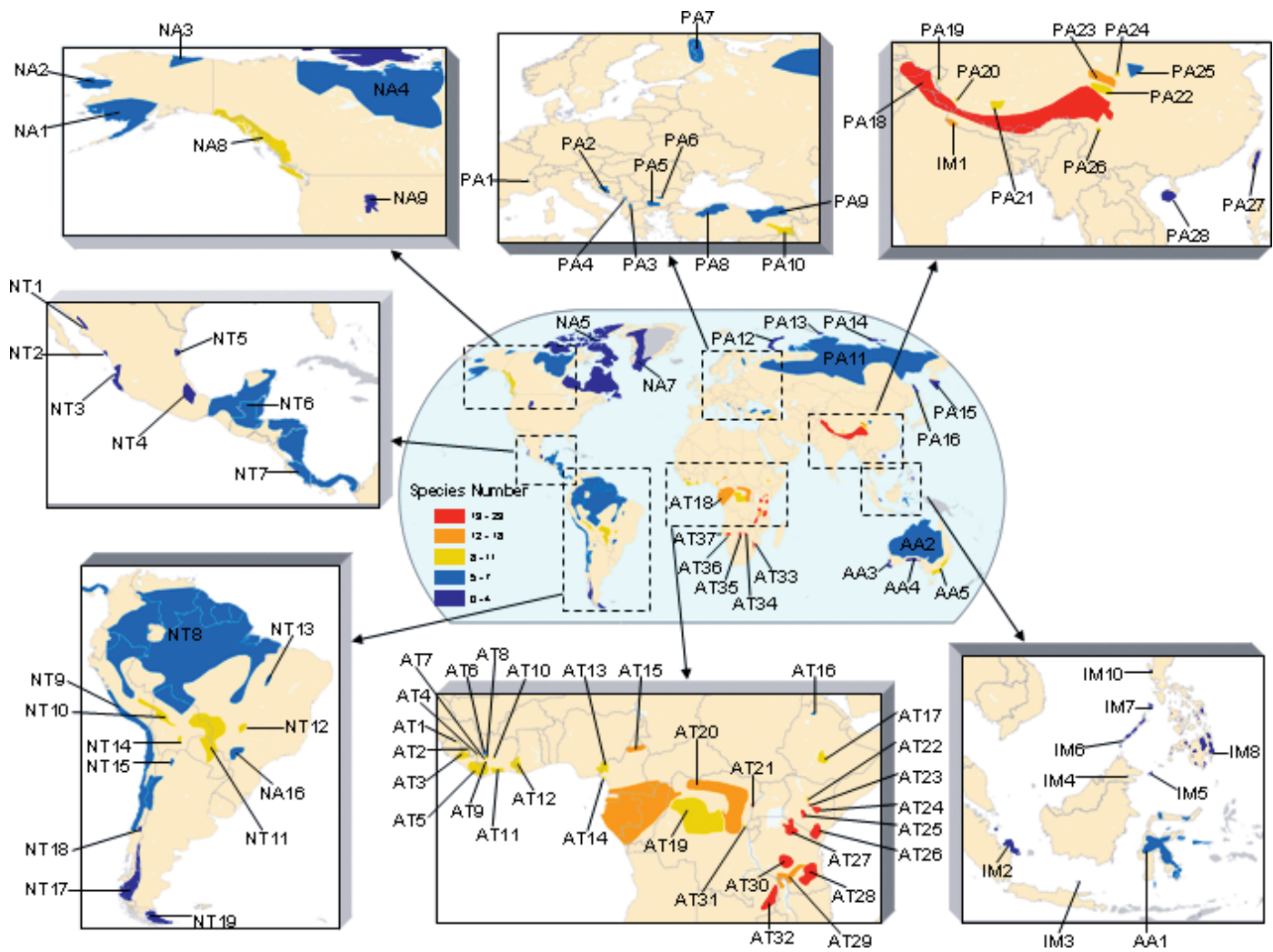
FIG. 1. —Intact large mammal faunas. Colored portions of the map indicate the number of species each intact large mammal area contains. Warm colors denote species-rich sites, whereas cool colors are less rich. The pink areas possessed large mammals in AD 1500 but no longer contained all of their former species. Gray areas did not possess large mammals historically (Antarctica would be gray but is not depicted). Note that the areas with highest mammal richness (East Africa and Indomalaya) have some of the lowest coverage of intact mammal faunas. Map numbers refer to Table 1 (AAxx = Australasia; ATxx = Afrotropics; IMxx = Indomalaya; NAxx = Nearctic; NTxx = Neotropics; PAxx = Palearctic).
