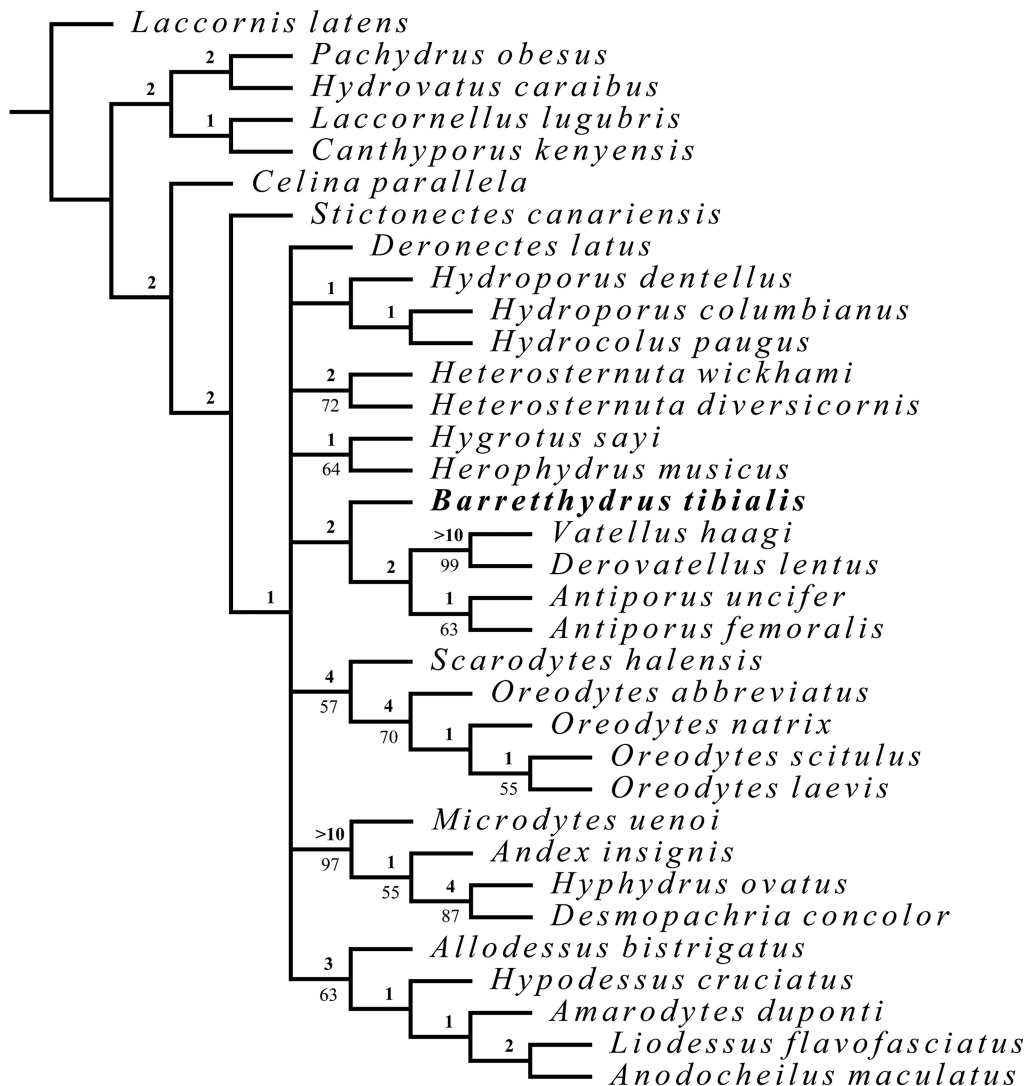
Fig. 20. Strict consensus cladogram obtained from the cladistic analysis of 34 terminal taxa of Hydroporinae, with Bremer support values indicated above branches and Bootstrap values higher than 50 indicated below branches.
