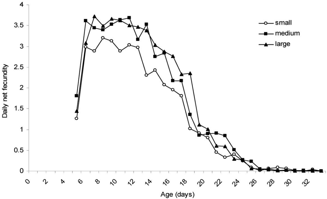
Fig. 2. Daily net fecundity of small, medium, and large Diachasmimorpha longicaudata females.
