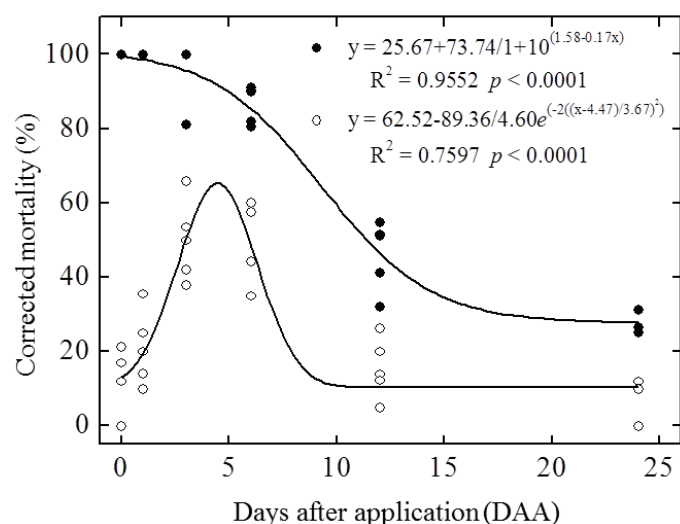
Fig. 4. Corrected mortality (Schneider-Orelli 1947) of Diaphorina citri adults exposed to residue on 'Valência' sweet orange seedlings treated with an aqueous emulsion of ethanol extract from Annona mucosa seeds — ESAM (●) — or the commercial limonoid-based bioinsecticide Azamax® 1.2 EC (○) used as a positive control, at different periods after application in a semi-field trial (greenhouse). The mortality levels were lower than 7.5% in the controls.
